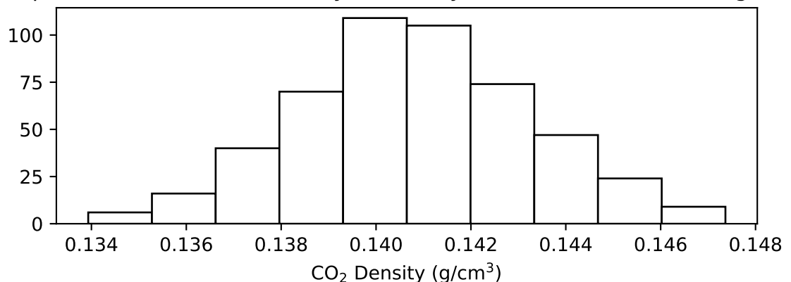
Input distribution CO 2 density: Normally-distributed, 1\sigma = 0.003 g/cm 3
