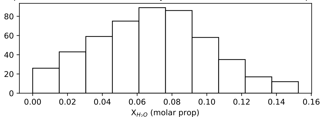
Input Distribution XH 2 O: Normally-distributed, 1\sigma = 0.034 molar prop
